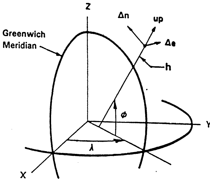
Figure Geocentric, Geodetic and Local Coordinates
