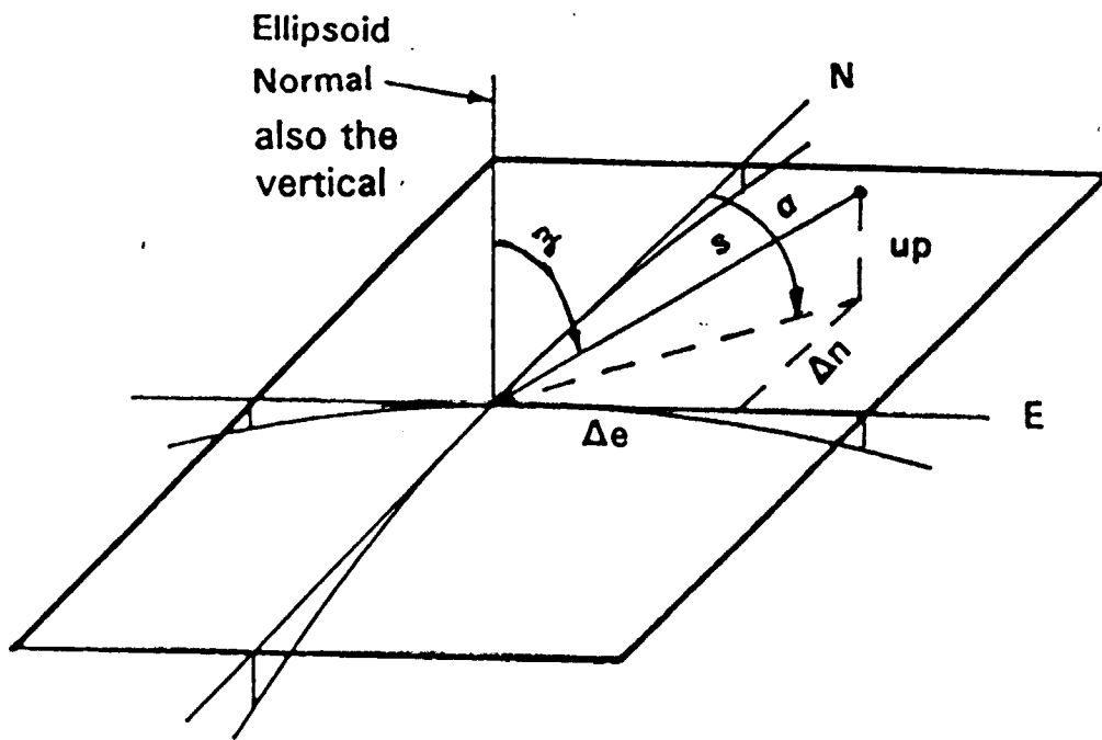
Figure Local Plane Coordinate System
