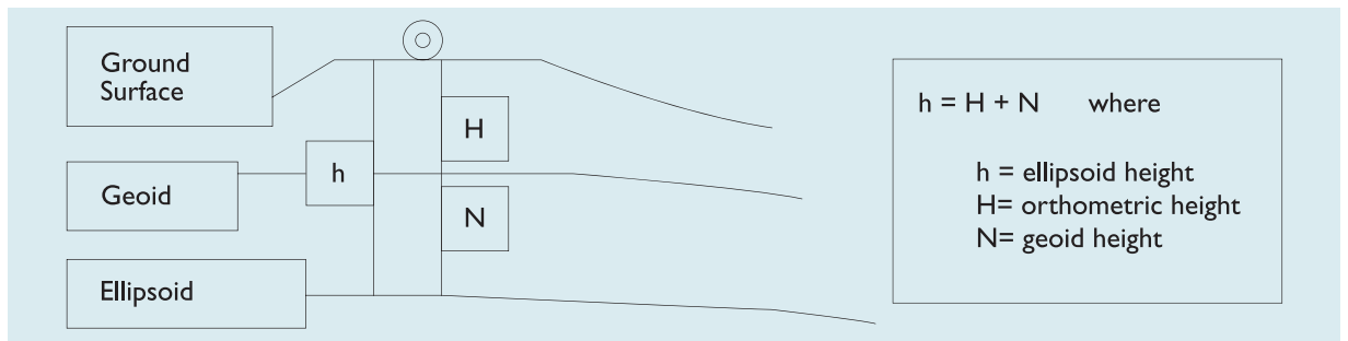
Figure 1, Relationship between ellipsoid height, orthometric height and geoid height.
