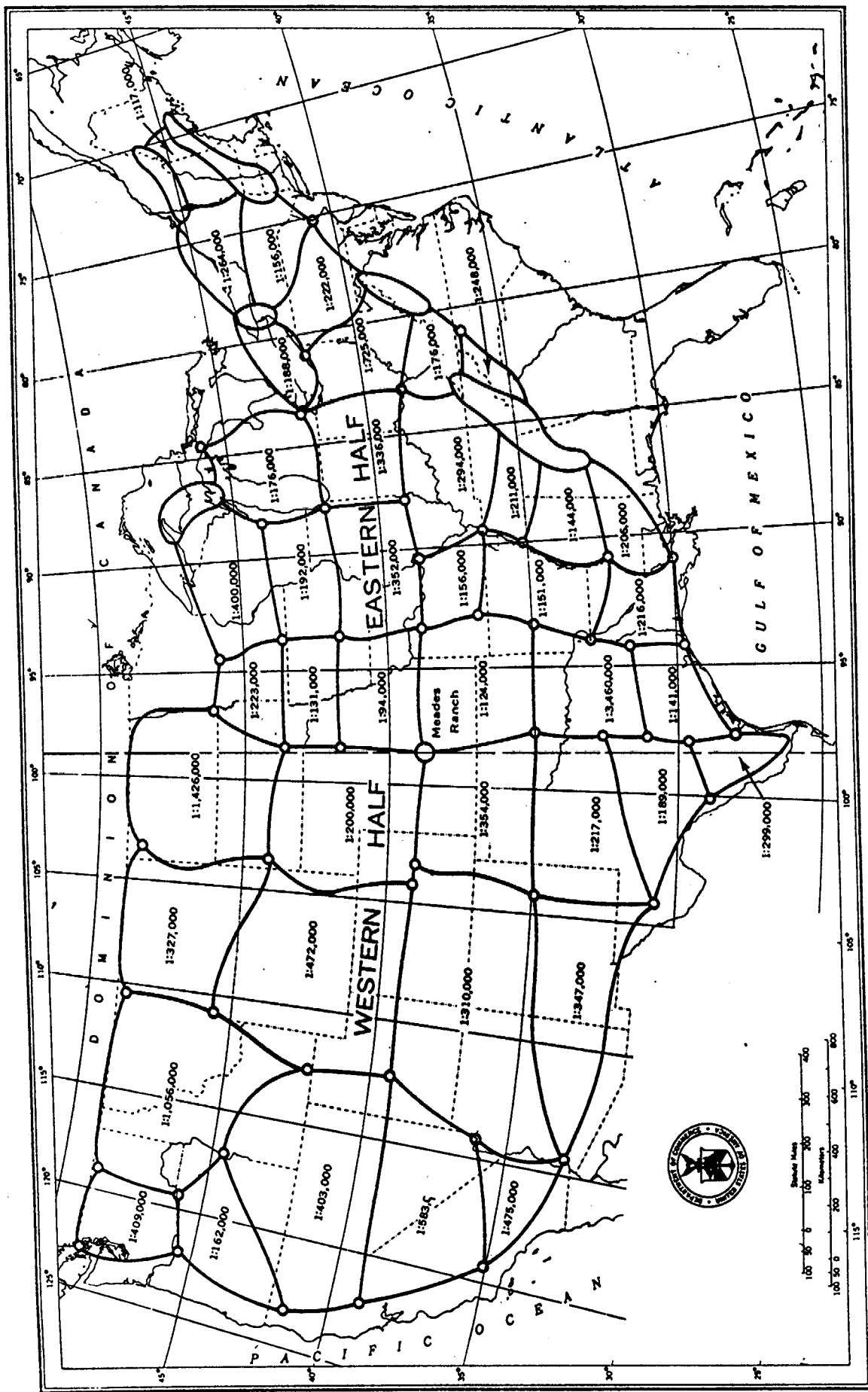
FIGURE 4 Adjustment closures for the North American 1927 Datum.
