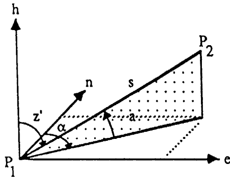
FIGURE 7.2 Reduced observations in the local geodetic coordinate system.
