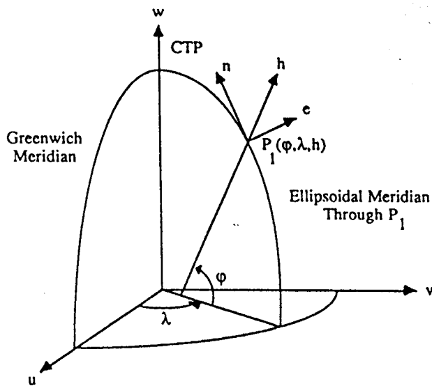
FIGURE 7.1 The local geodetic coordinate system.
