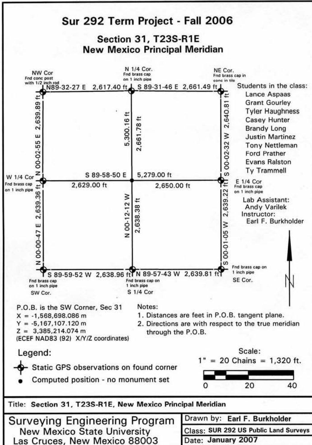
FIG 2 Plat of Survey – Section 31, T23S-R1E, New Mexico Principal Meridian
